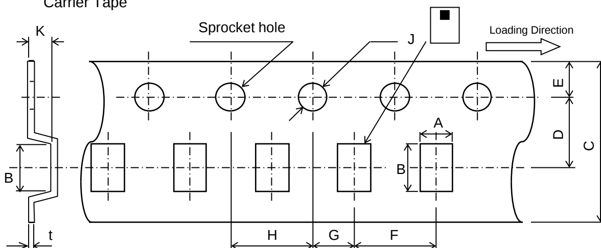
Carrier Tape
