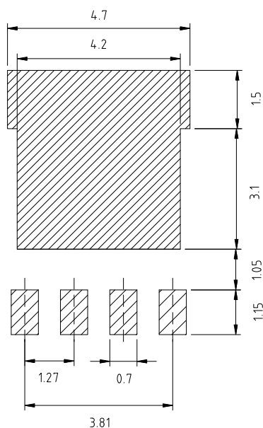
Figure 19. LFPK 5x6 recommended footprint (dimensions in mm)
