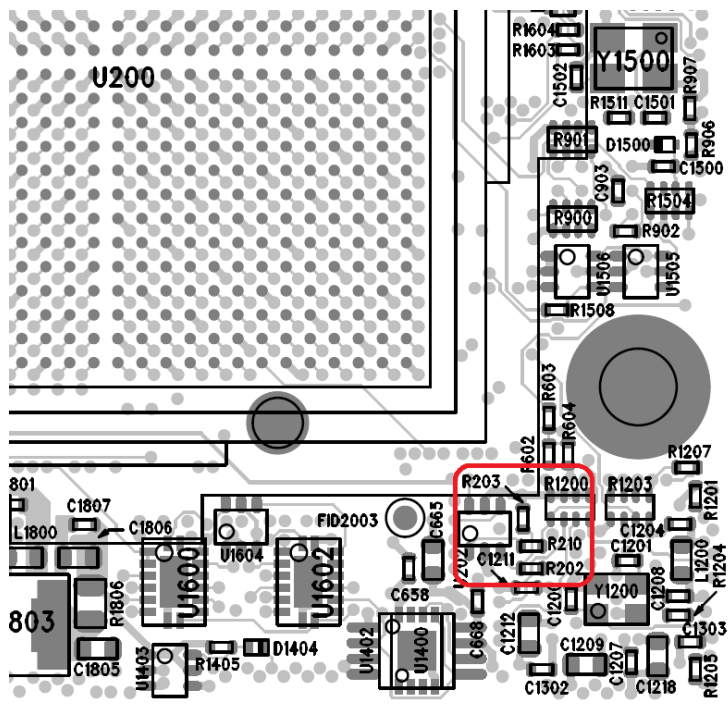
Figure 12: Pull-Up During Configuration (PUDC) Resistors - Assembly Drawing Top View (lower right part)
