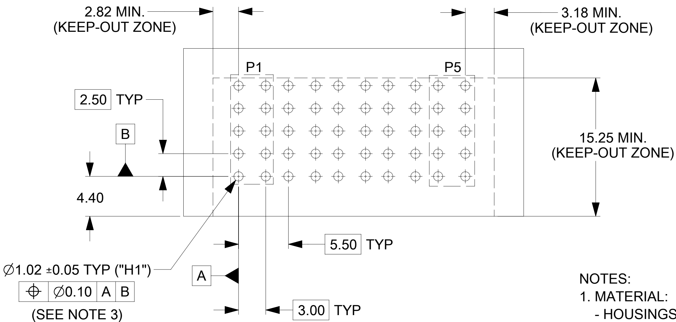
RECOMMENDED PCB LAYOUT AND KEEP-OUT ZONE
