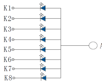
LED(B/L) CIRCUIT
