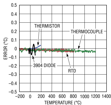
Typical Temperature Error Contribution
