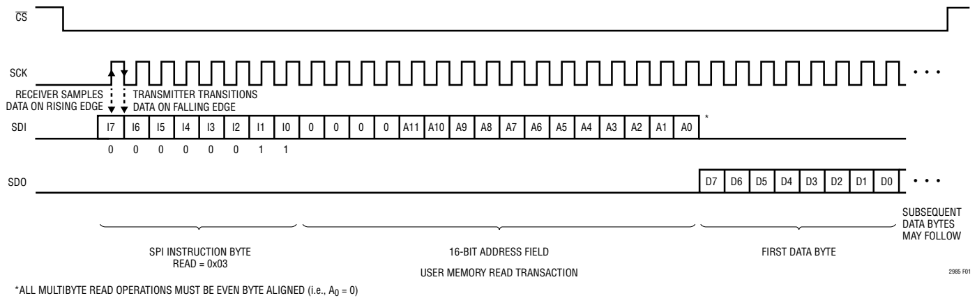
Figure 1. Memory Read Operation
