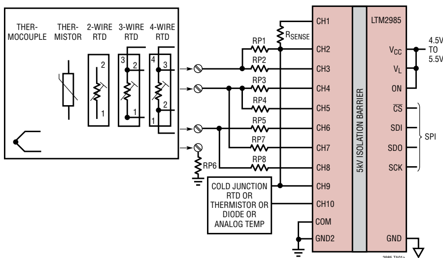
Universal Isolated Temperature Measurement System
