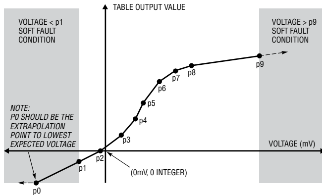
Figure 57. Direct ADC Table Example
