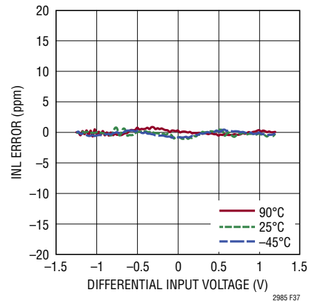
Figure 56. Integral Nonlinearity as a Function of Temperature at V_{CC2} = 5.25V
