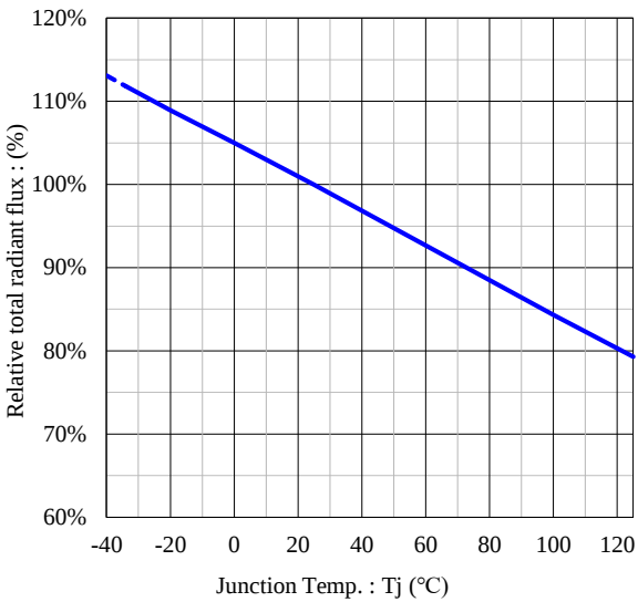
Junction temp. vs. Relative total radiant flux
