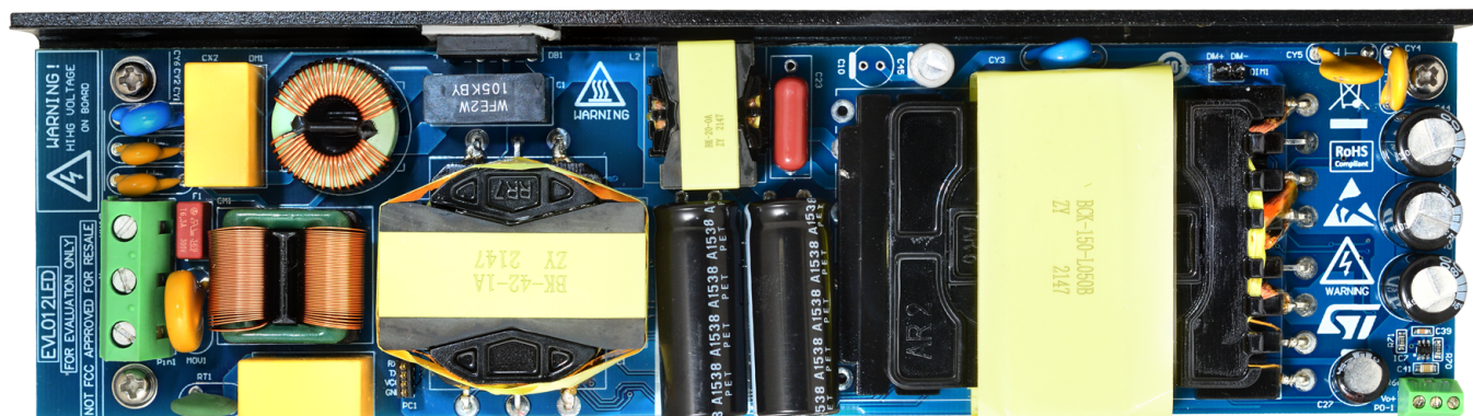
Figure 1. EVL012LED board
