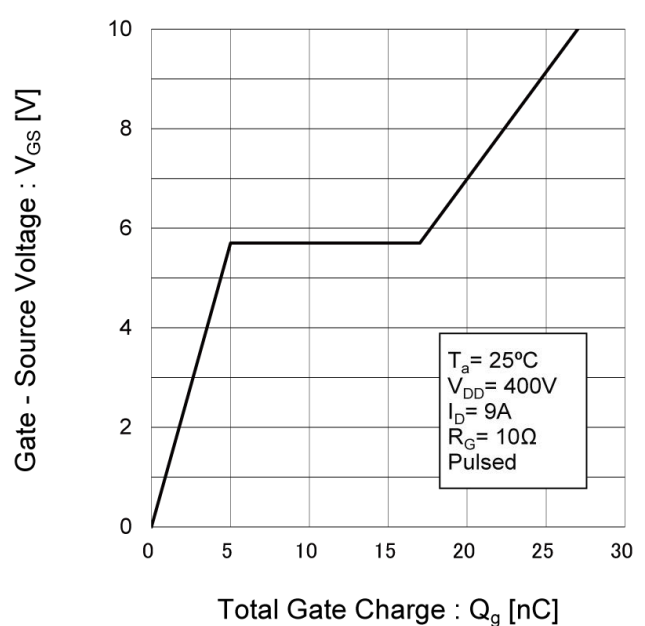
Fig.16 Gate Charge
