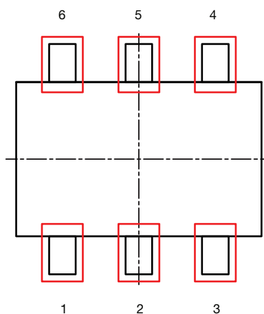
TSOP-6L
