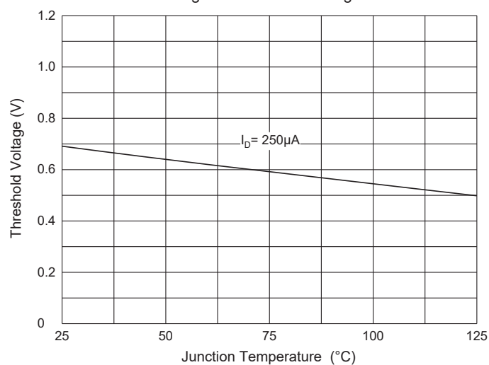
Fig. 6 - Threshold Voltage
