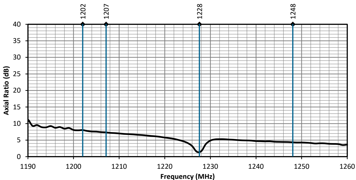
Figure 9. ANT-GNCP-C25L12100 Antenna Axial Ratio, L2 Band
