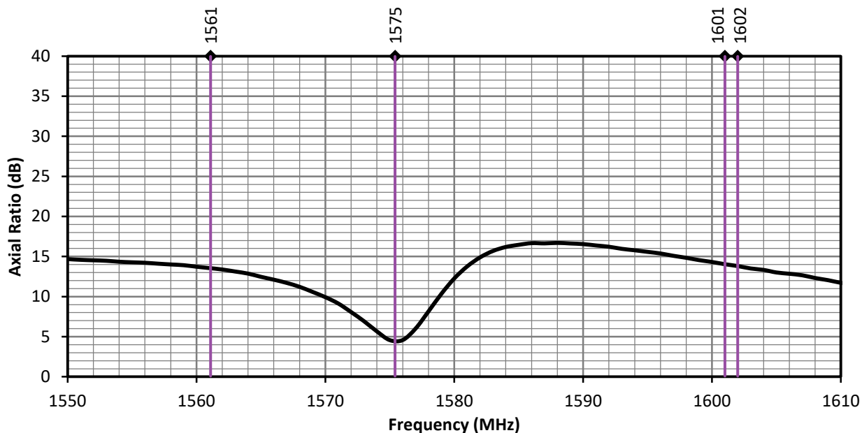
Figure 8. ANT-GNCP-C25L12100 Antenna Axial Ratio, L1 Band
