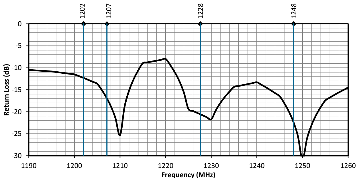
Figure 5. ANT-GNCP-C25L12100 Return Loss, L2 Band
