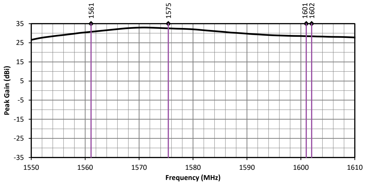
Figure 6. ANT-GNCP-C25L12100 Peak Gain, L1 Band
