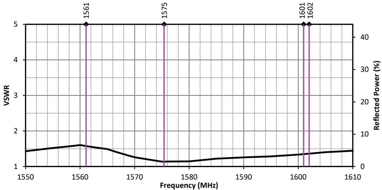
Figure 2. ANT-GNCP-C25L12100 VSWR, L1 Band
