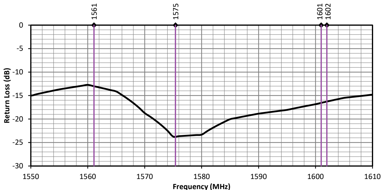
Figure 4. ANT-GNCP-C25L12100 Return Loss, L1 Band
