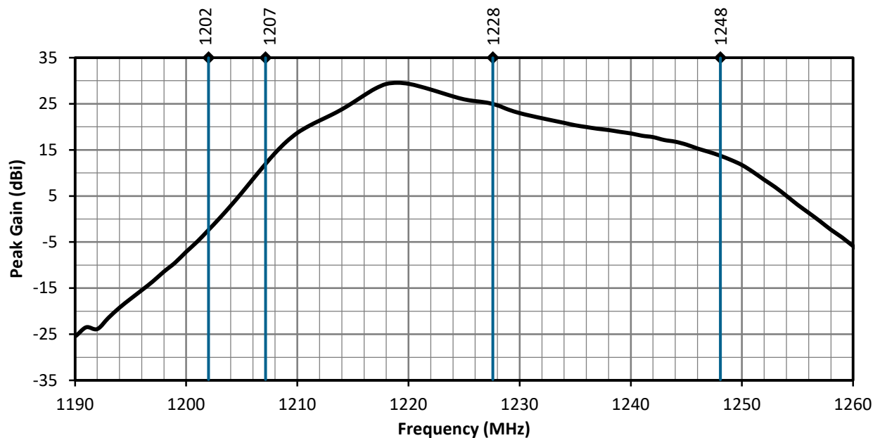
Figure 7. ANT-GNCP-C25L12100 Peak Gain, L2 Band
