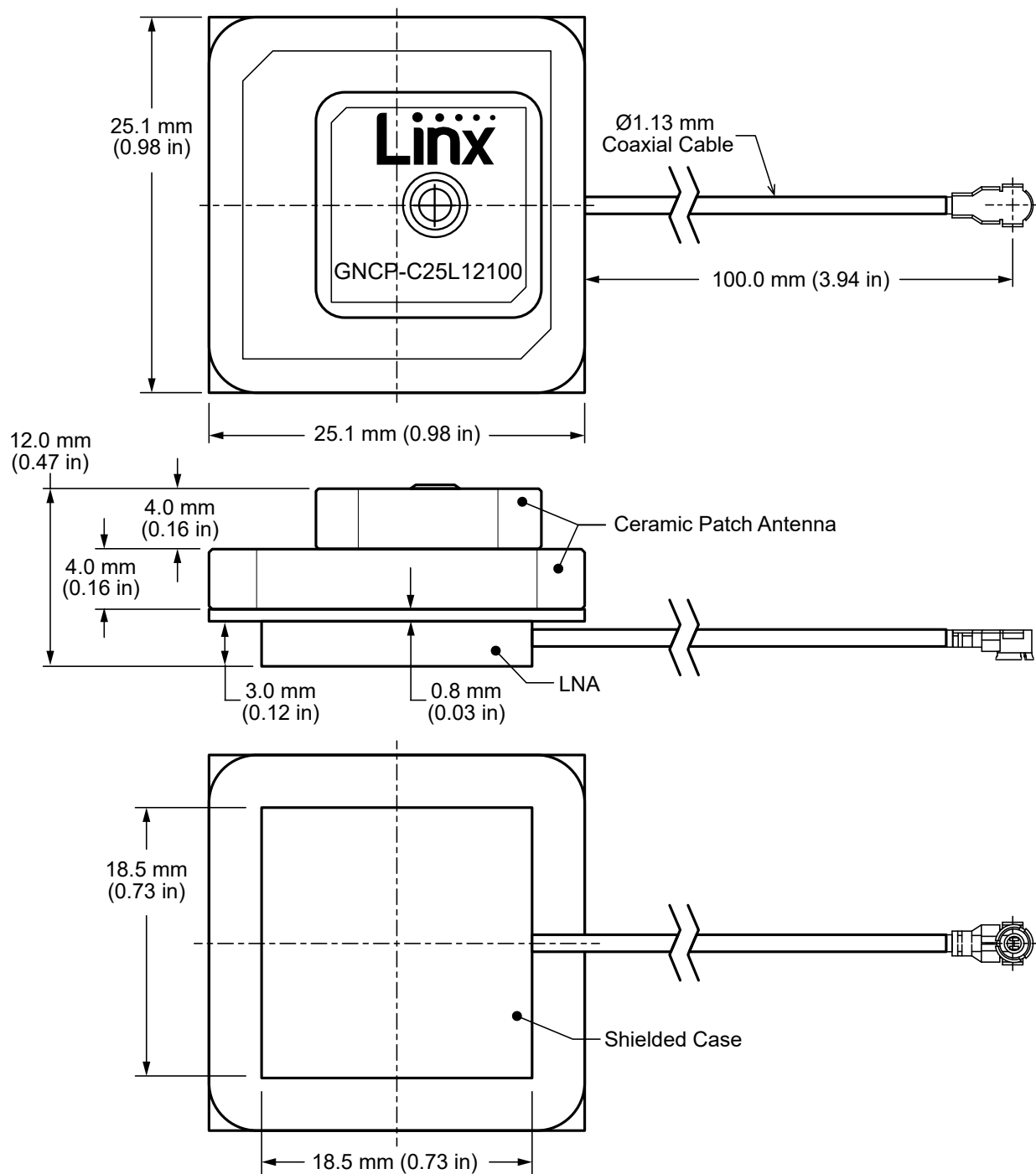
Figure 1. ANT-GNCP-C25L12100 Antenna Dimensions
