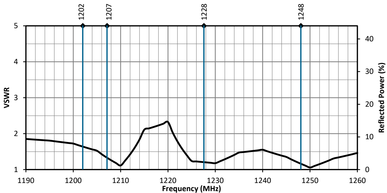
Figure 3. ANT-GNCP-C25L12100 VSWR, L2 Band
