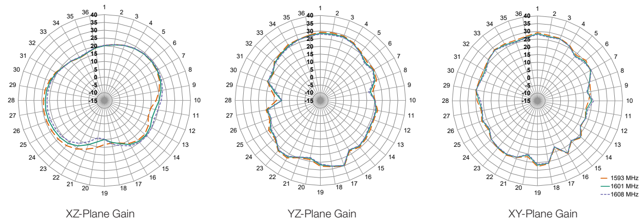
Figure 10. ANT-GNCP-C25L12100 Radiation Patterns
