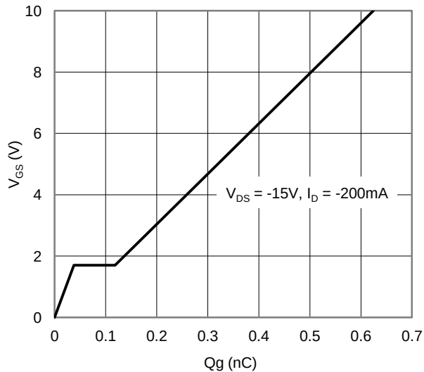
Figure 23. Gate Charge
