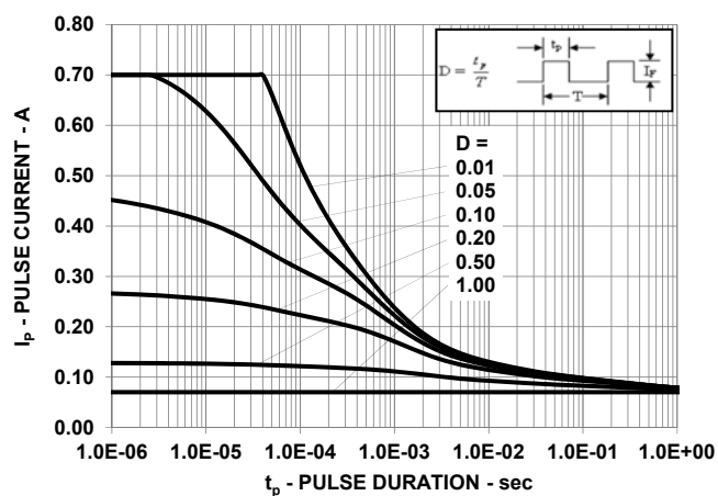
Figure 8: Pulse handling capability at T_S < 42^{\circ}\text{C} . Derated based on R_{\theta JA} = 460^{\circ}\text{C/W}
