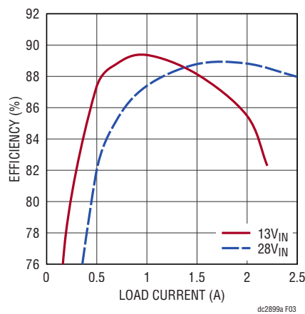
Figure 3. DC2899A Output Efficiency vs Load Current ( T_A = 25^{\circ}\text{C} )
