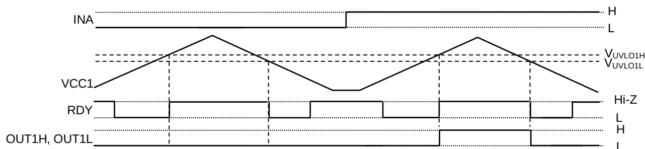
Figure 56. Input-side UVLO Function Operation Timing Chart
