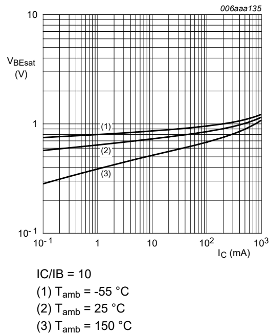
Fig. 10. BC817-25QB: Base-emitter saturation voltage as a function of collector current; typical values
