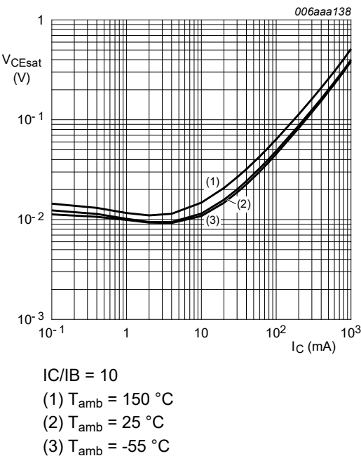
Fig. 11. BC817-25QB: Collector-emitter saturation voltage as a function of collector current; typical values
