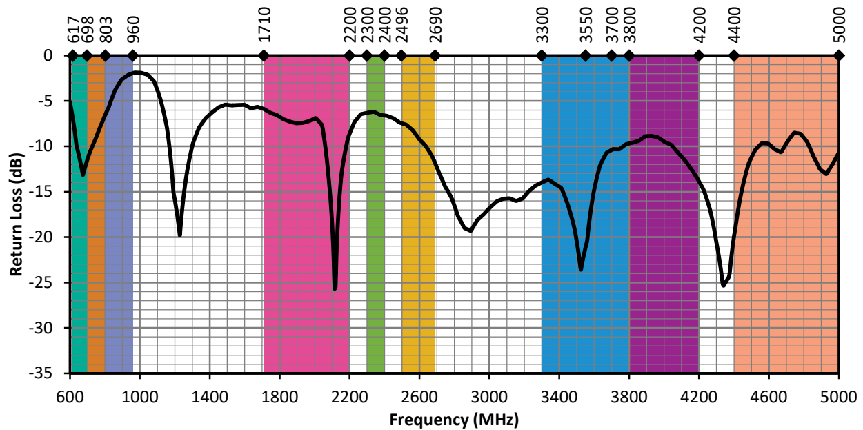
Figure 12. ANT-5GW-IPW1-NP Return Loss, Center of Ground Plane
