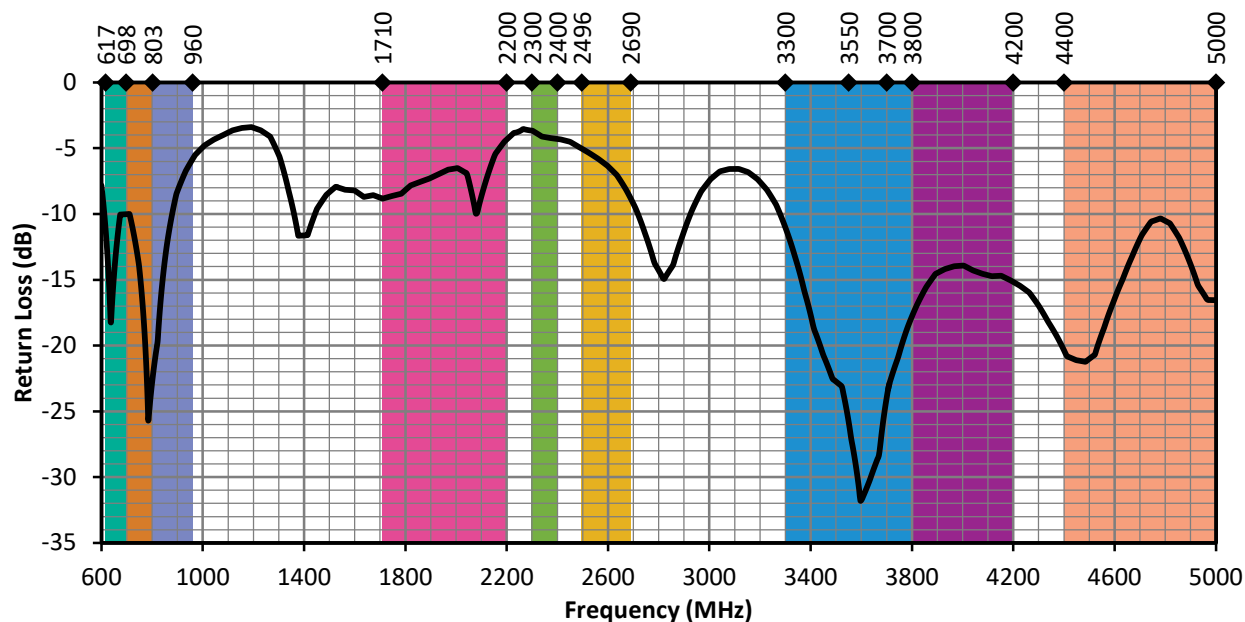
Figure 5. ANT-5GW-IPW1-NP Return Loss, Free Space
