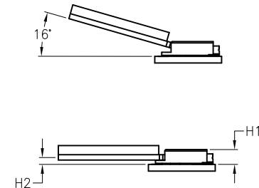
MATING CONDITION
