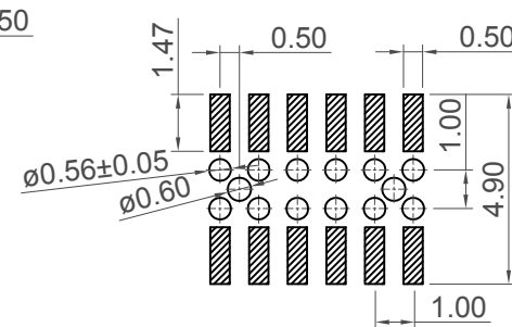
Recommended PCB Layout For Bottom Entry Solder Area
