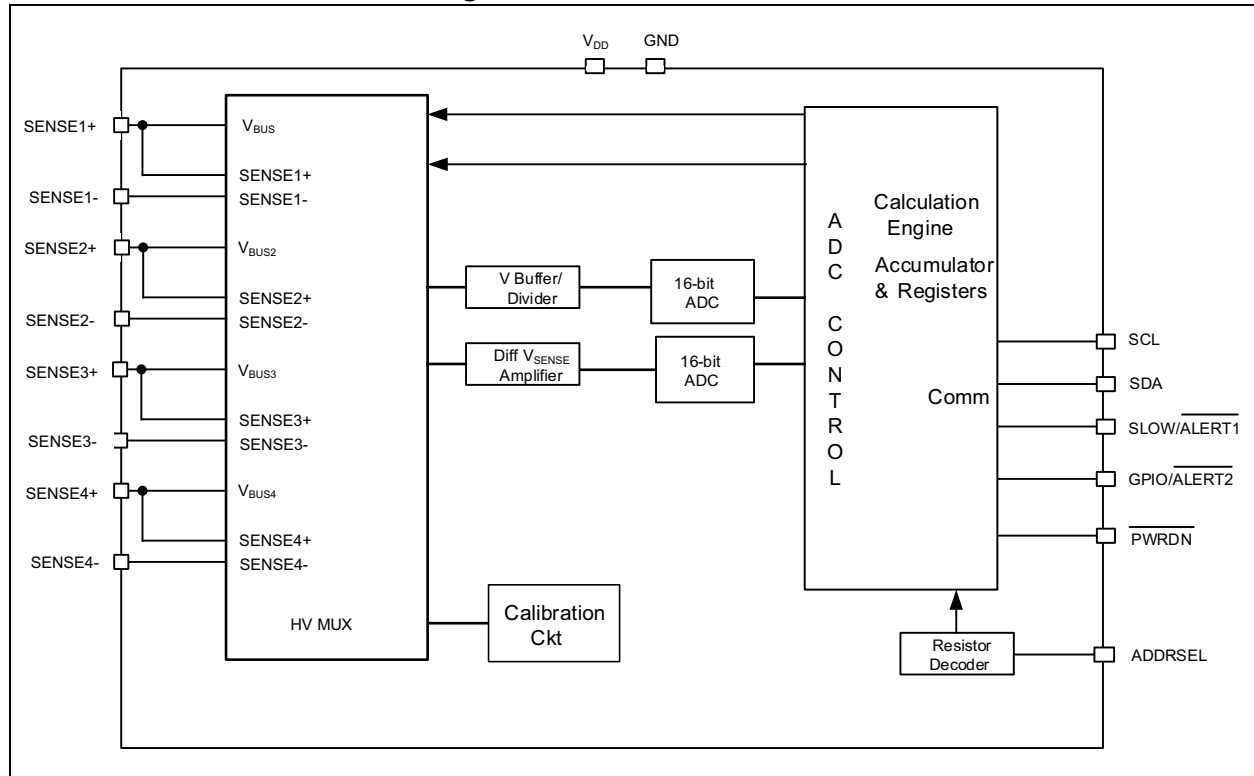
PAC195X-1 Functional Block Diagram
