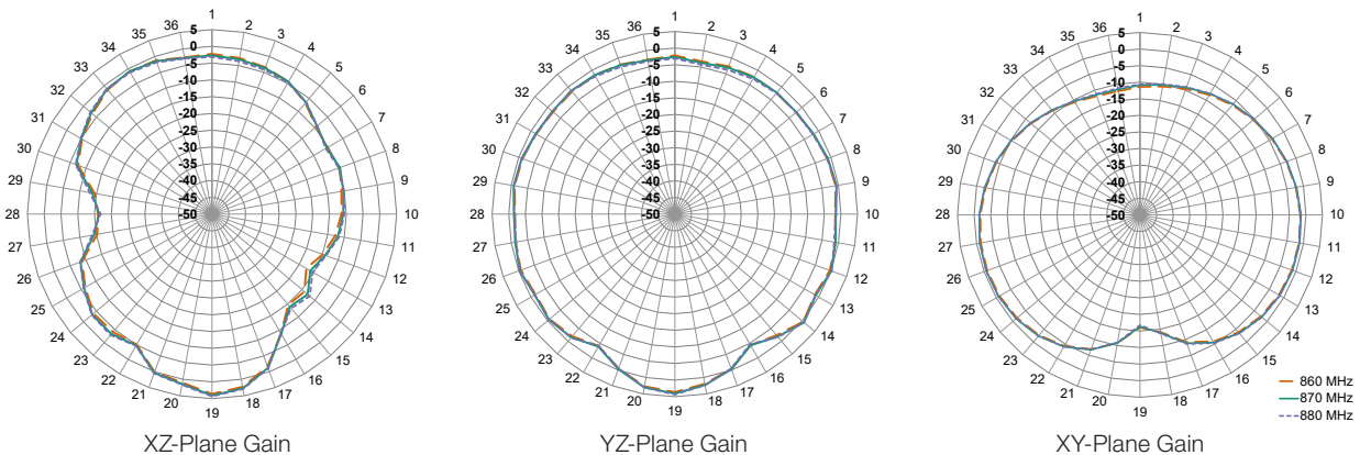
Figure 9. Radiation Patterns for ANT-868-NUB-ccc Antenna, Edge of ground Plane
