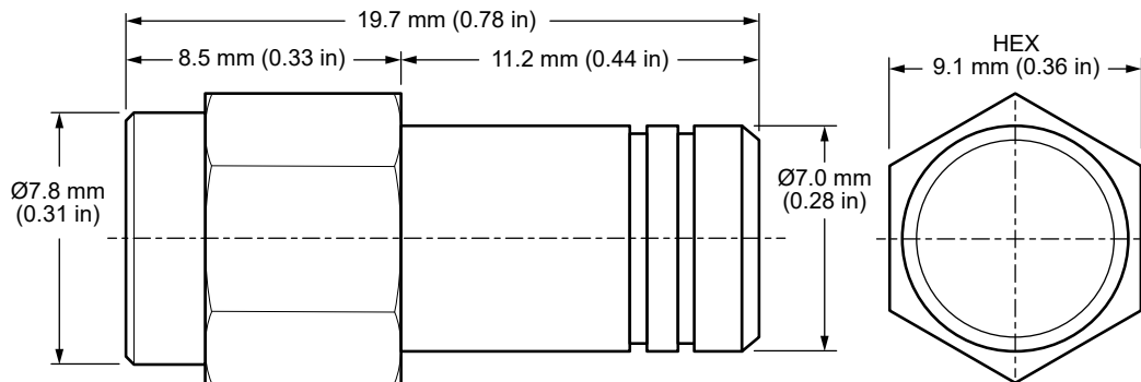
Figure 1. ANT-868-NUB-ccc Antenna Dimensions
