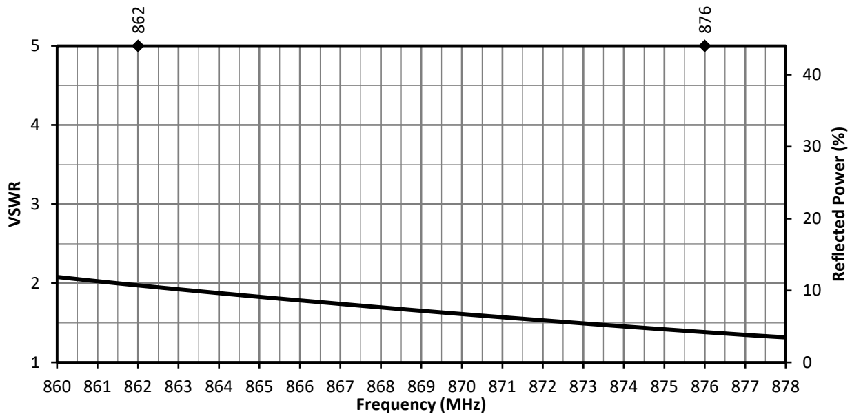
Figure 11. VSWR for ANT-868-NUB-ccc Antenna in Free Space
