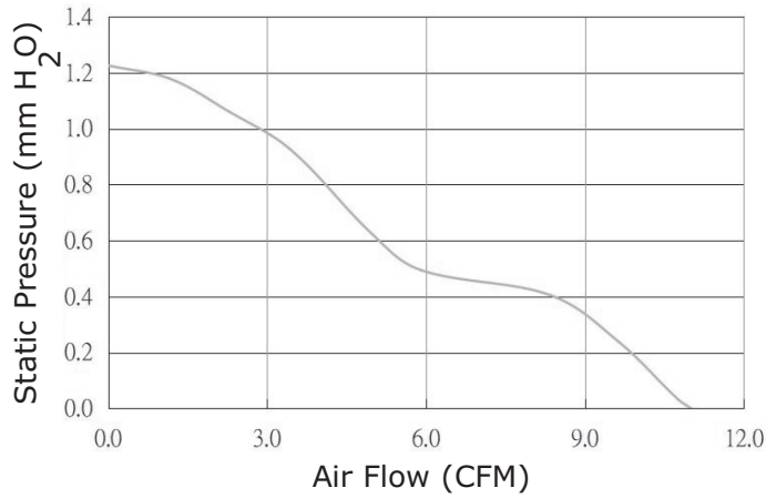
CFM-6015BF-245-332
