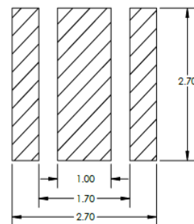
Recommended PCB Solder Pad
