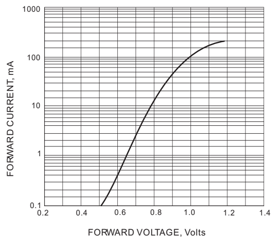
FIG. 1-TYPICAL FORWARD CHARACTERISTIC
