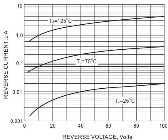
FIG. 2-TYPICAL REVERSE CHARACTERISTICS
