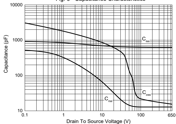
Fig. 6 - Capacitance Characteristics
