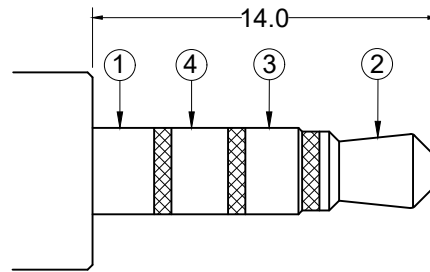
Ø3.5 MATE PLUG
