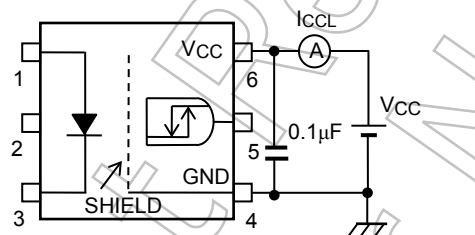
TEST CIRCUIT 3: I_{CCL}
