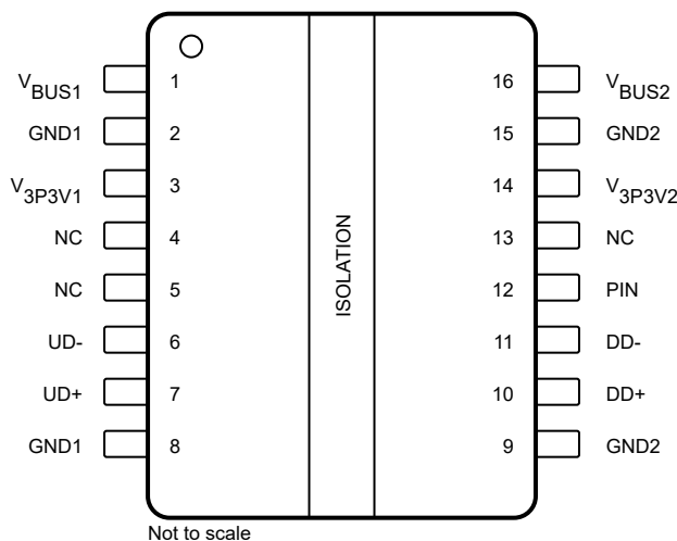
Figure 3-1. ISOUSB111DWX Full/Low Speed Isolated USB Repeater Pin Configuration
