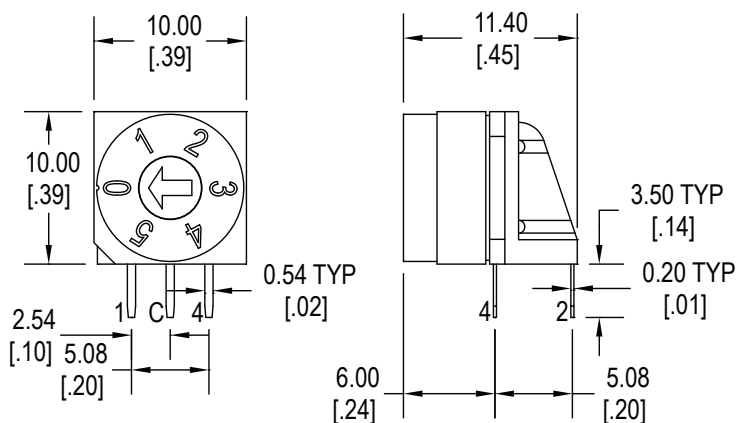
VB Terminals
