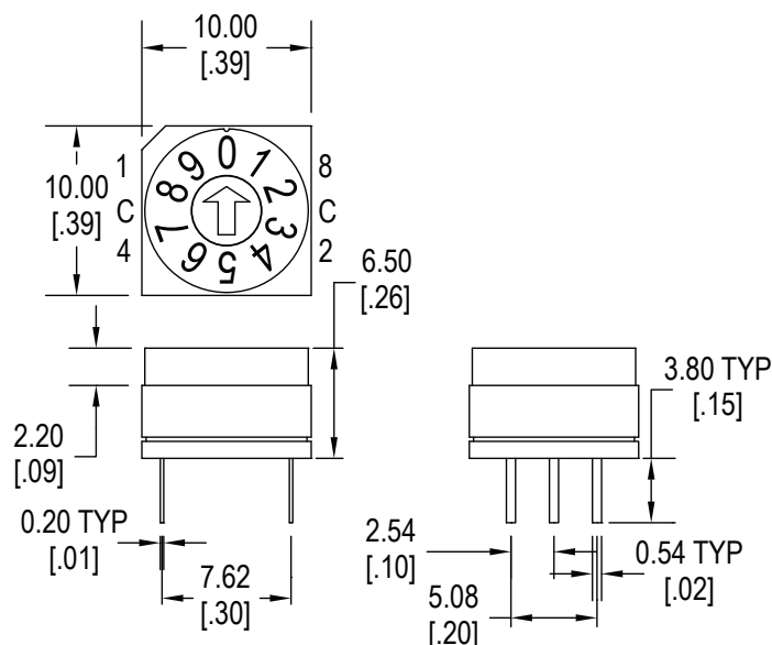
T Terminals
