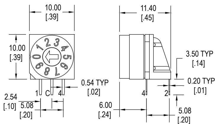
VB Terminals
