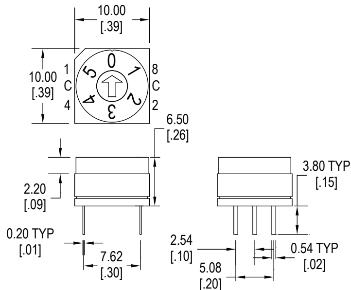
T Terminals
