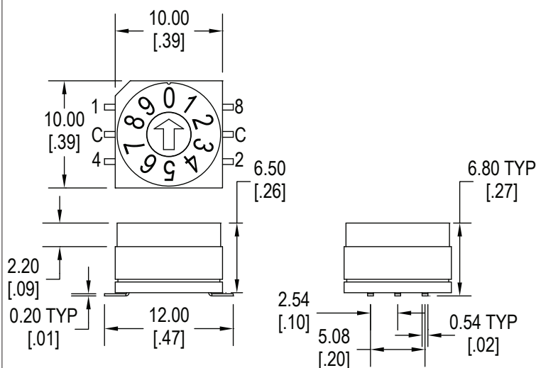
G Terminals
