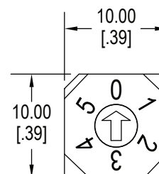
A - Octagonal
