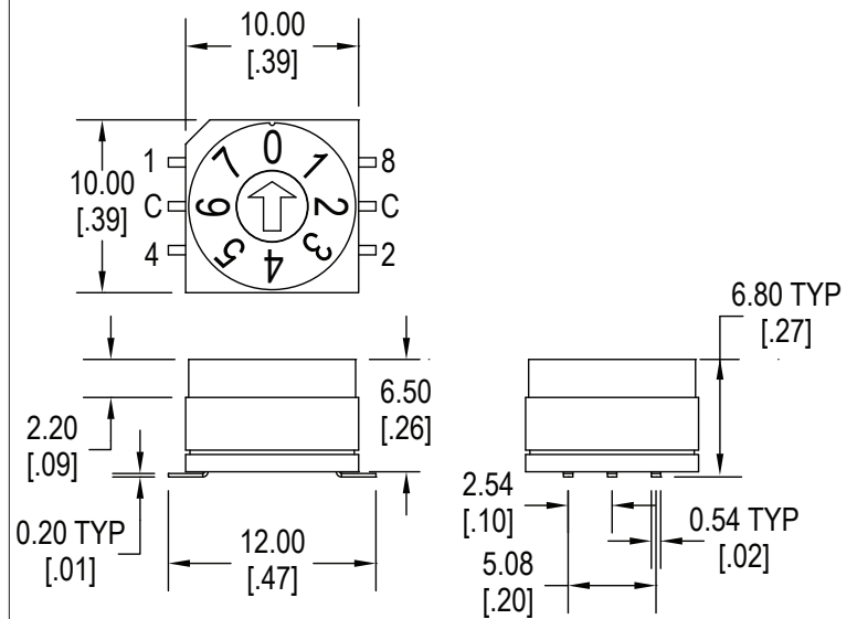
G Terminals
