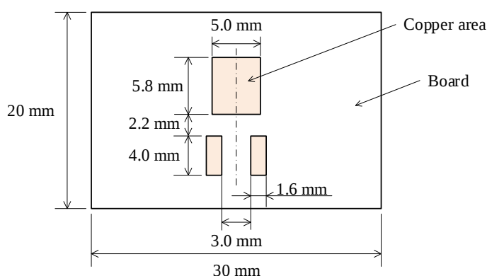
Figure 2. Glass-epoxy Board
