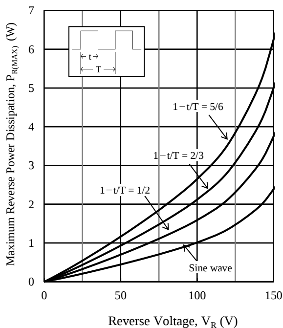
Figure 6. P_{R(MAX)} vs. V_R ( T_J = 150 °C)
