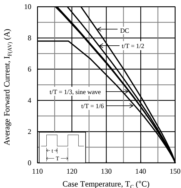
Figure 3. I_{F(AV)} vs. T_C ( T_J = 150 °C, V_R = 0 V)
