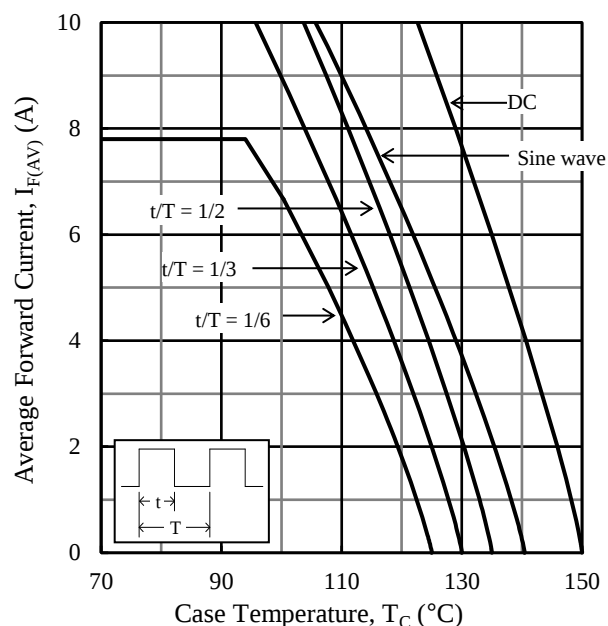
Figure 4. I_{F(AV)} vs. T_C ( T_J = 150 °C, V_R = 150 V)
