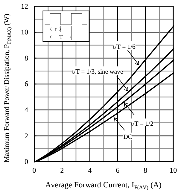
Figure 5. P_{F(MAX)} vs. I_{F(AV)} ( T_J = 150 °C)
