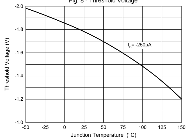
Fig. 8 - Threshold Voltage
