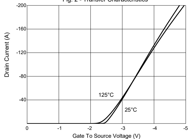
Fig. 2 - Transfer Characteristics
