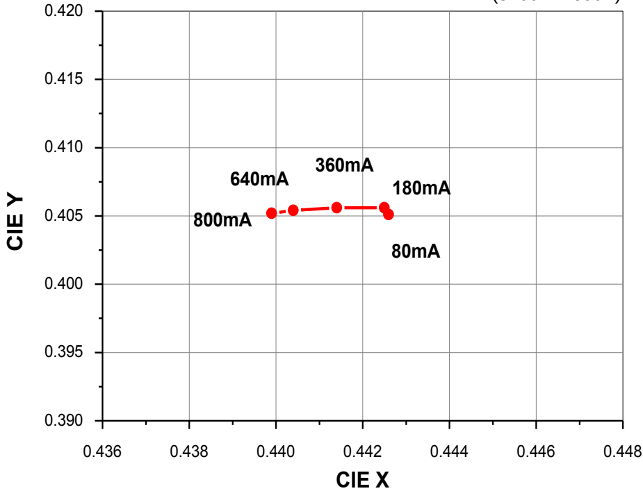
Fig 5. Forward Current vs. CIE X, Y Shift , T_j=25^{\circ}\text{C} (CRI80) (3700K~2600K)
