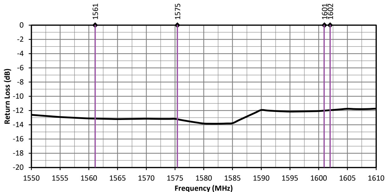
Figure 3. ANT-GNCP-C185L160 Return Loss
