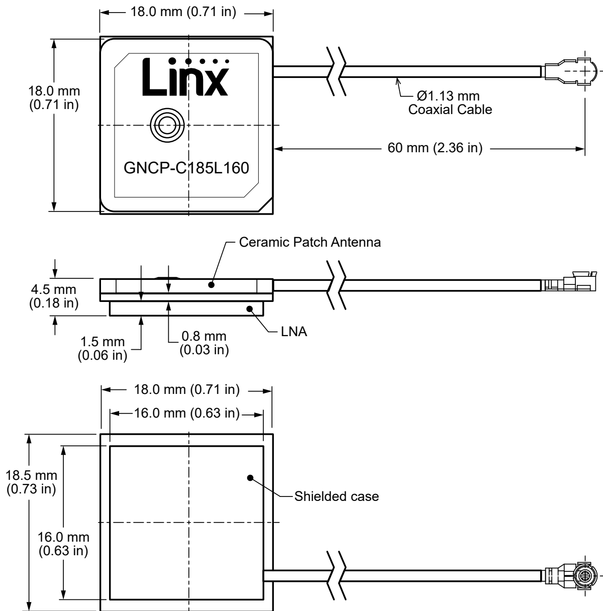
Figure 1. ANT-GNCP-C185L160 Antenna Dimensions
