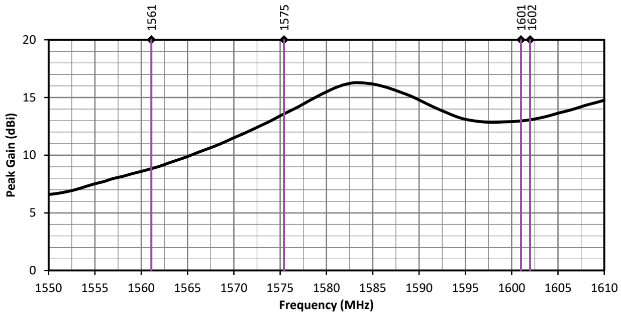
Figure 4. ANT-GNCP-C185L160 Peak Gain
