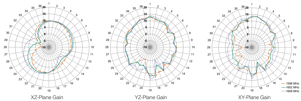
Figure 6. ANT-GNCP-C185L160 Radiation Patterns
