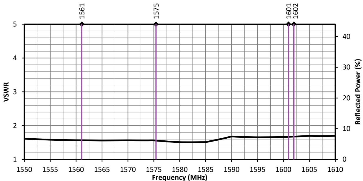
Figure 2. ANT-GNCP-C185L160 VSWR
