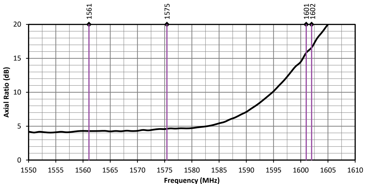
Figure 5. ANT-GNCP-C185L160 Antenna Axial Ratio
