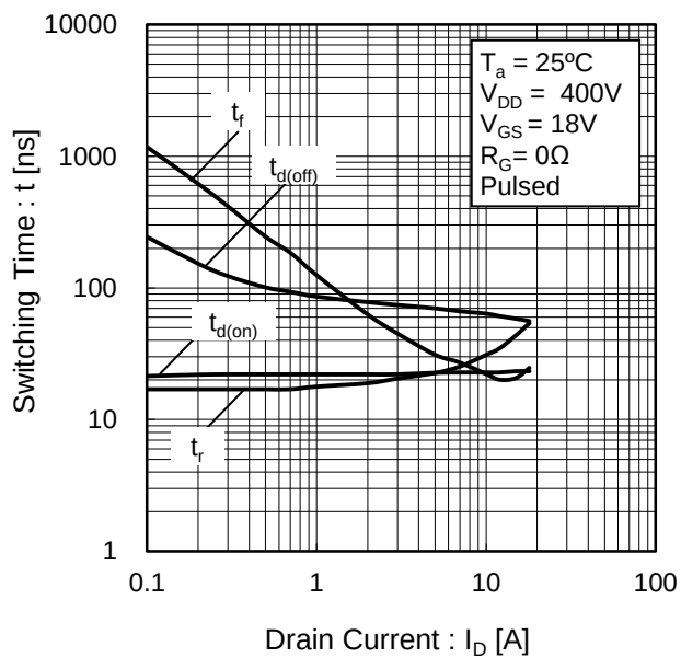
Fig.17 Switching Characteristics
