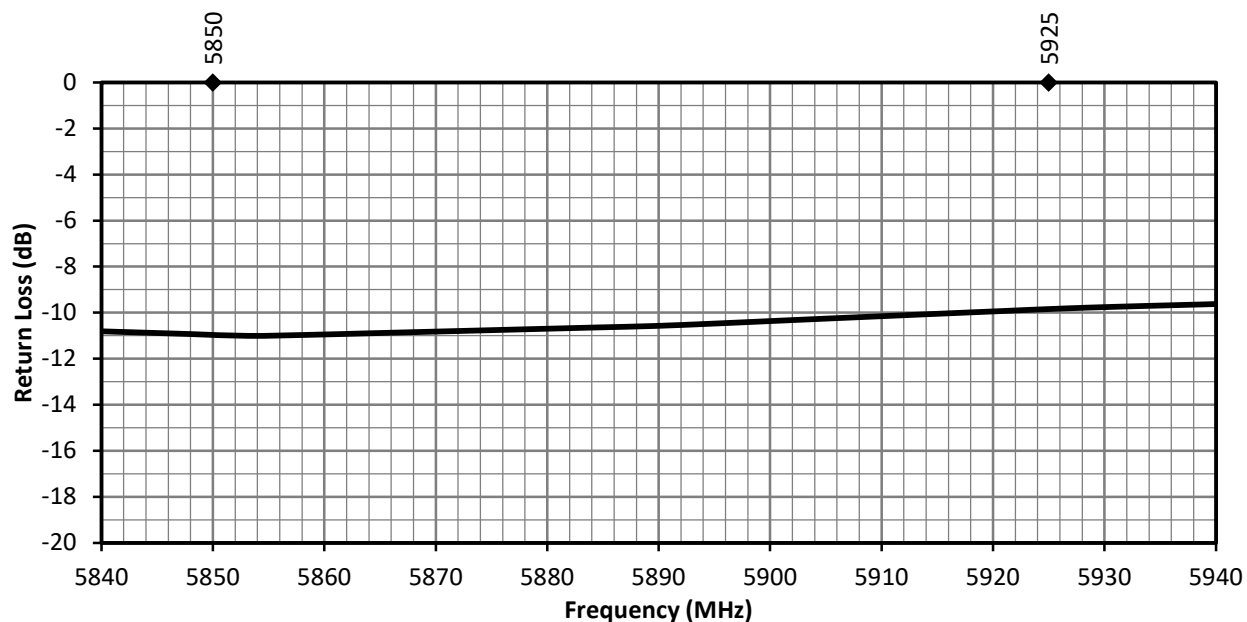
Figure 12. ANT-V2X-IPW1-NP Antenna Return Loss, Center of Ground Plane
