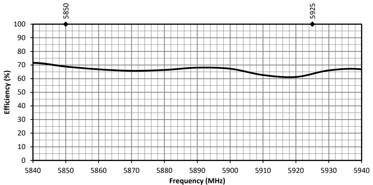
Figure 8. ANT-V2X-IPW1-NP Antenna Radiation Efficiency, Free Space
