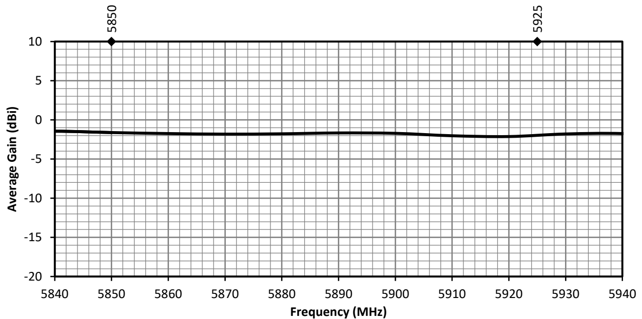
Figure 7. ANT-V2X-IPW1-NP Antenna Average Gain, Free Space
