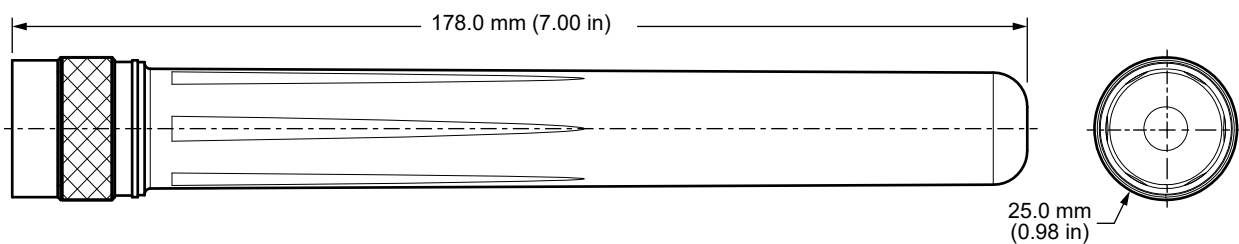
Figure 1. ANT-V2X-IPW1-NP Antenna Dimensions
