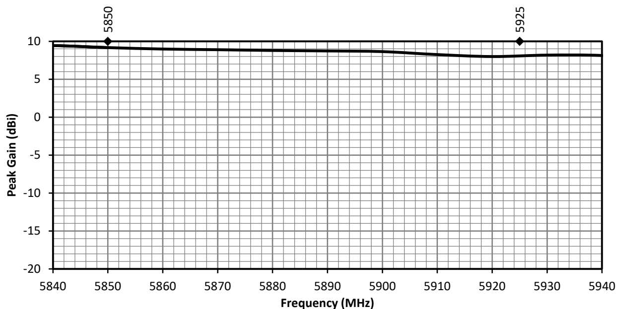
Figure 13. ANT-V2X-IPW1-NP Antenna Peak Gain, Center of Ground Plane
