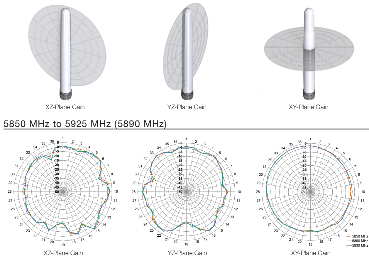
Figure 9. Radiation Patterns for ANT-V2X-IPW1-NP Antenna, Free Space
