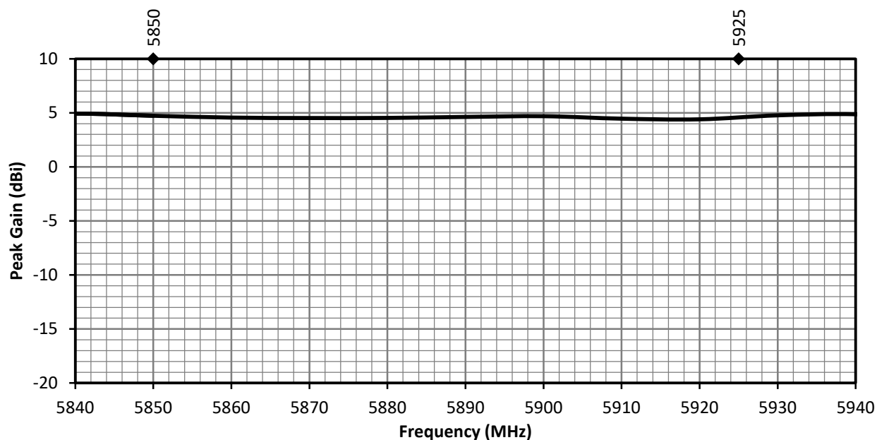
Figure 6. ANT-V2X-IPW1-NP Antenna Peak Gain, Free Space
