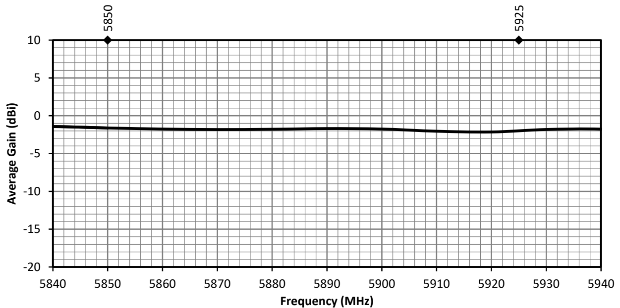
Figure 14. ANT-V2X-IPW1-NP Antenna Average Gain, Center of Ground Plane
