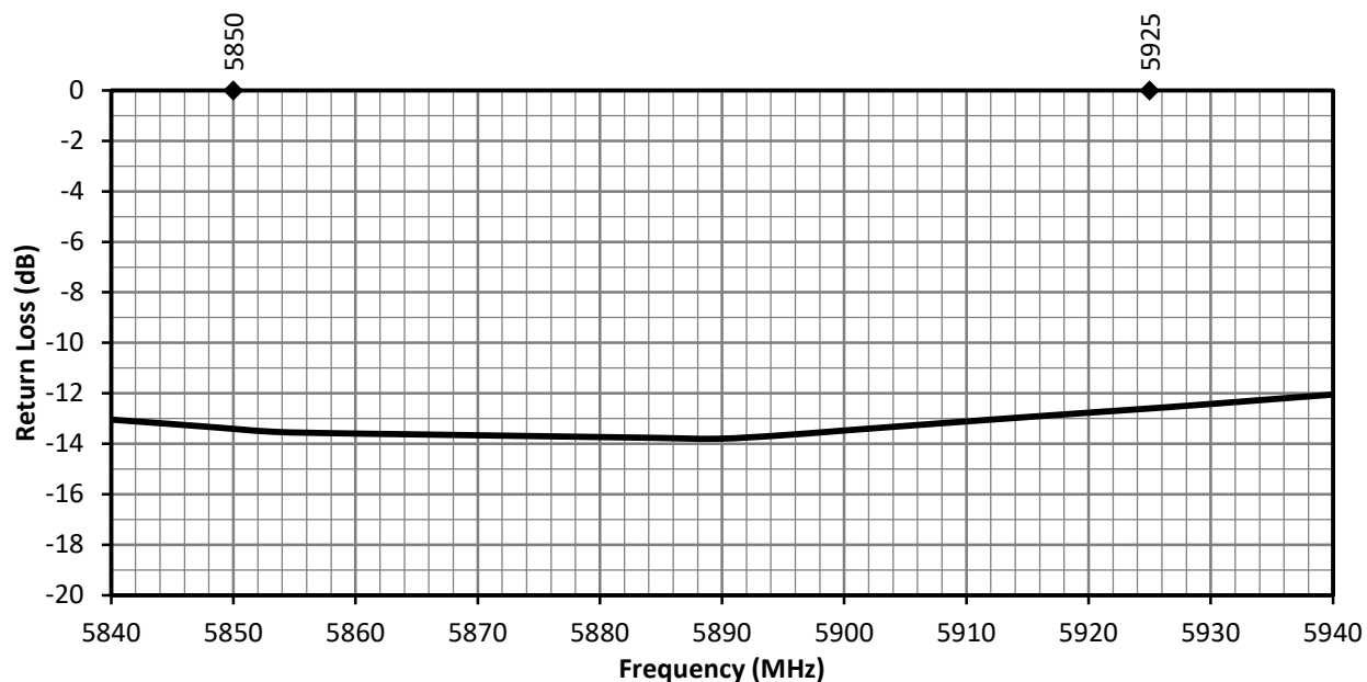
Figure 5. ANT-V2X-IPW1-NP Antenna Return Loss, Free Space
