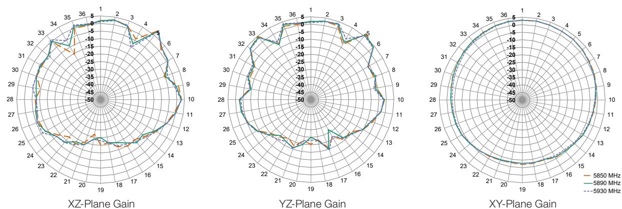
Figure 16. Radiation Patterns for ANT-V2X-IPW1-NP Antenna, Center of Ground Plane
