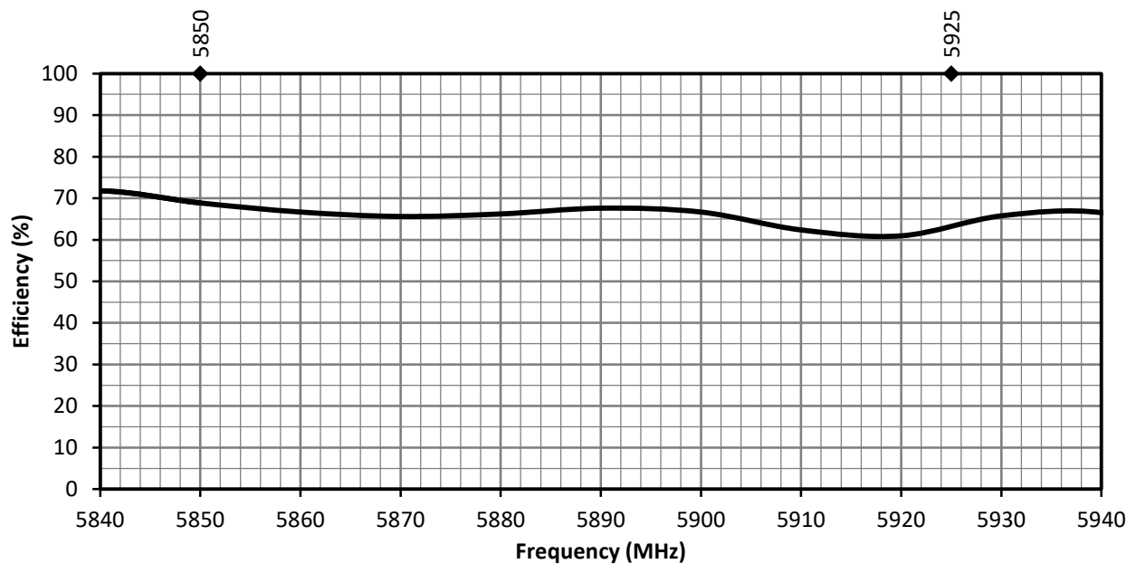
Figure 15. ANT-V2X-IPW1-NP Antenna Radiation Efficiency, Center of Ground Plane
