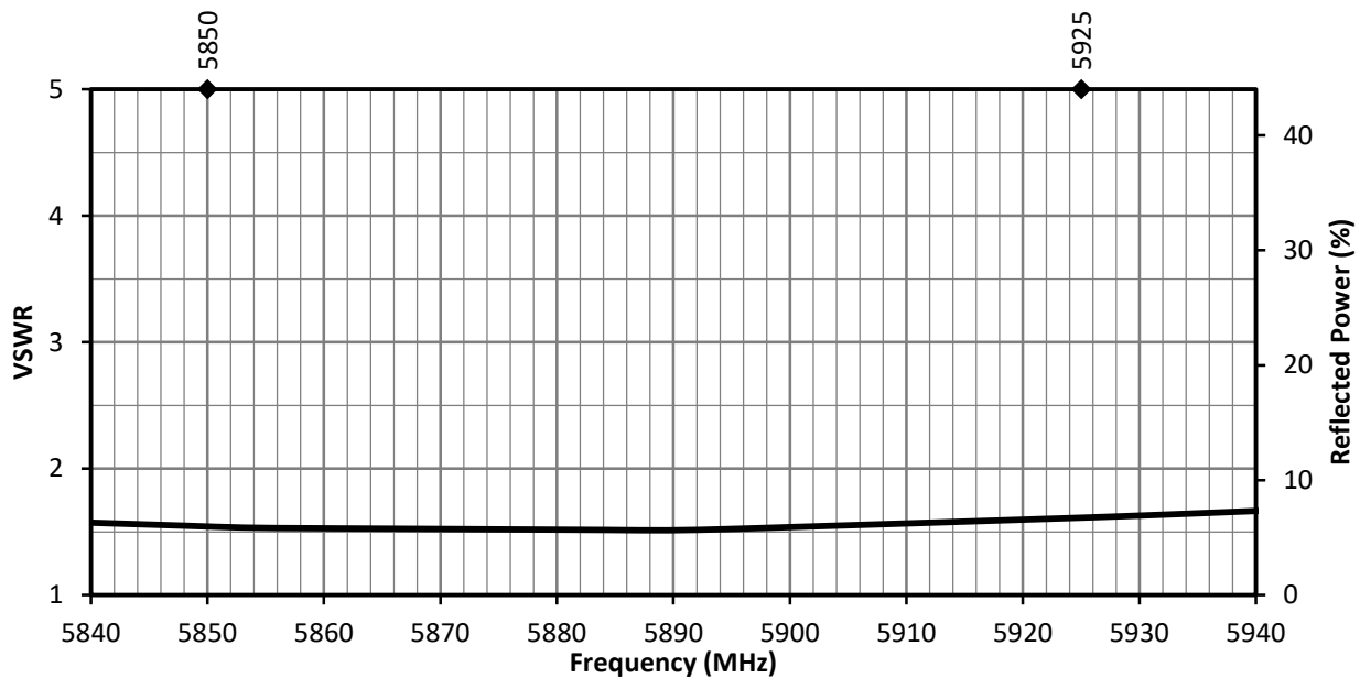
Figure 3. ANT-V2X-IPW1-NP Antenna VSWR, Free Space
