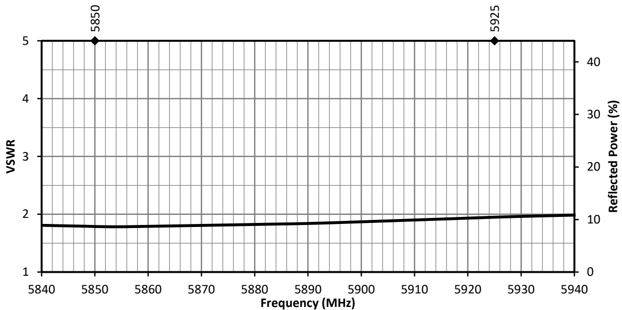
Figure 11. ANT-V2X-IPW1-NP Antenna VSWR, Center of Ground Plane
