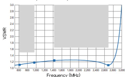
VSWR (Low-Band)
