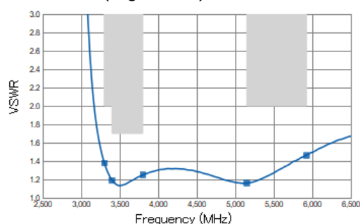
VSWR (High-Band)
