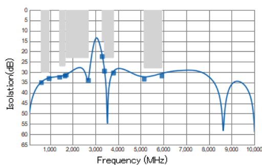
Isolation
