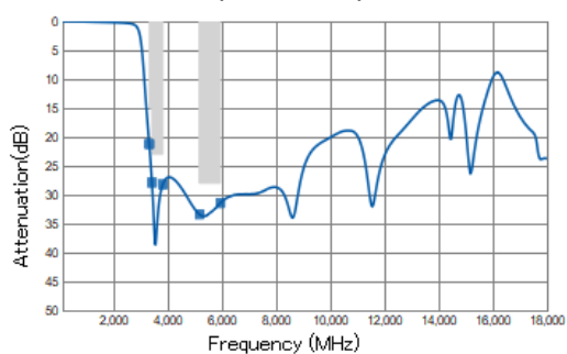
Attenuation (Low-Band)
