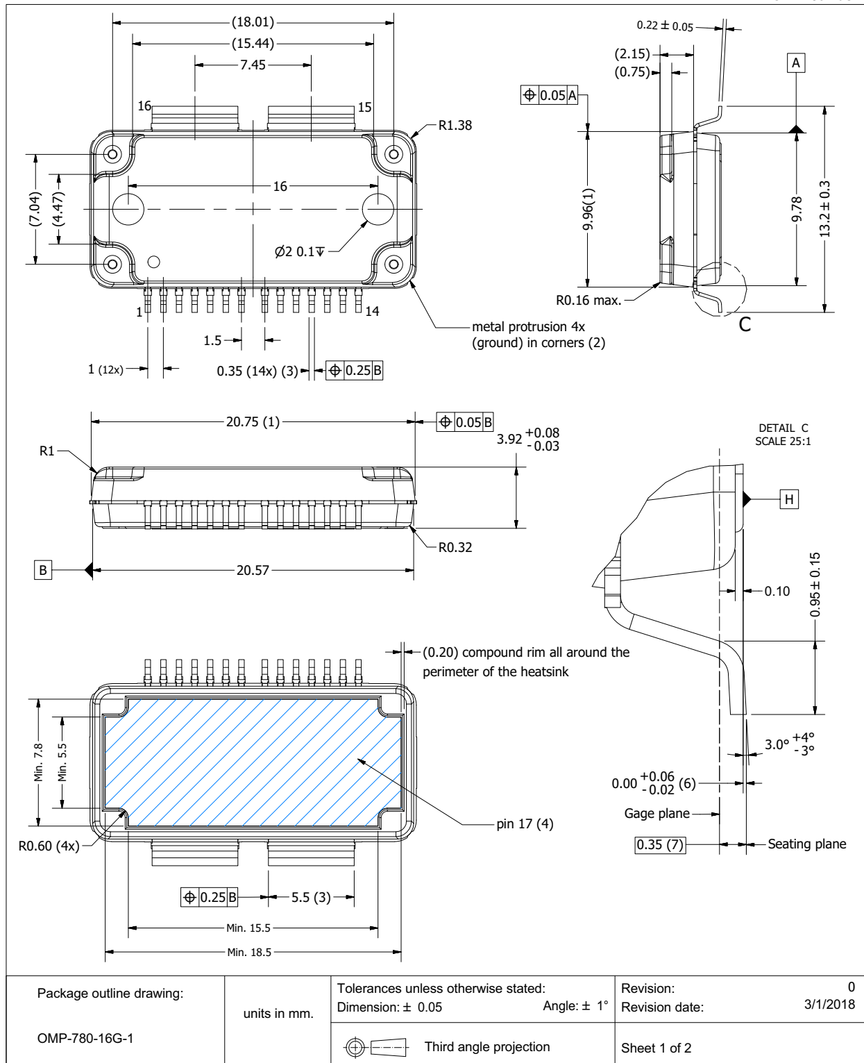
Fig 17. Package outline OMP-780-16G-1 (sheet 1 of 2)
