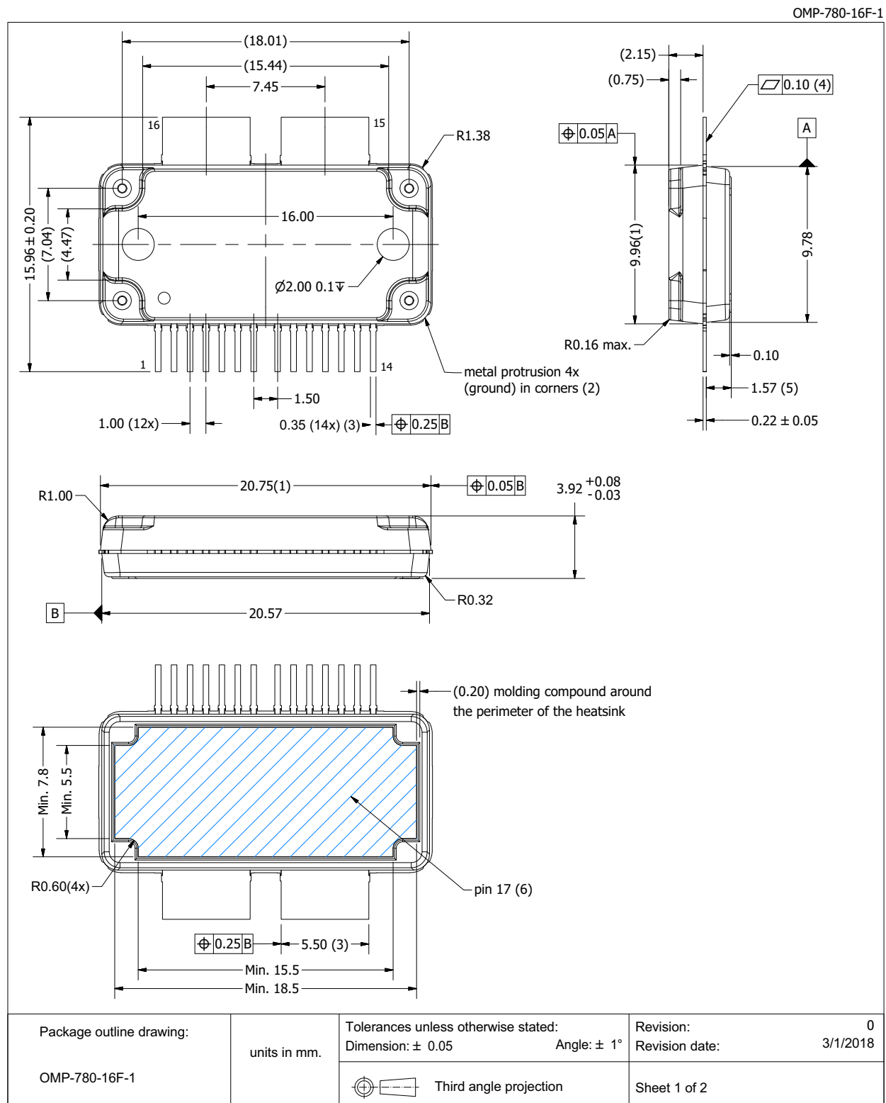
Fig 15. Package outline OMP-780-16F-1 (sheet 1 of 2)
