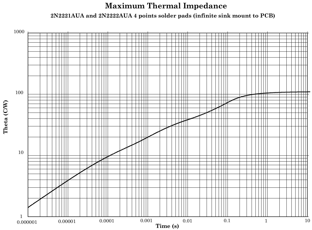
FIGURE 15. Thermal impedance graph ( R_{\theta JSP(1S)} ) for 2N2221AUA and 2N2222AUA.
