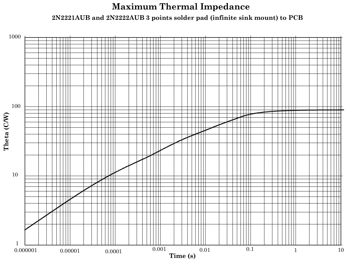
FIGURE 16. Thermal impedance graph ( R_{\theta JSP(S)} ) for 2N2221AUB and UBN and 2N2222AUB and UBCN.
