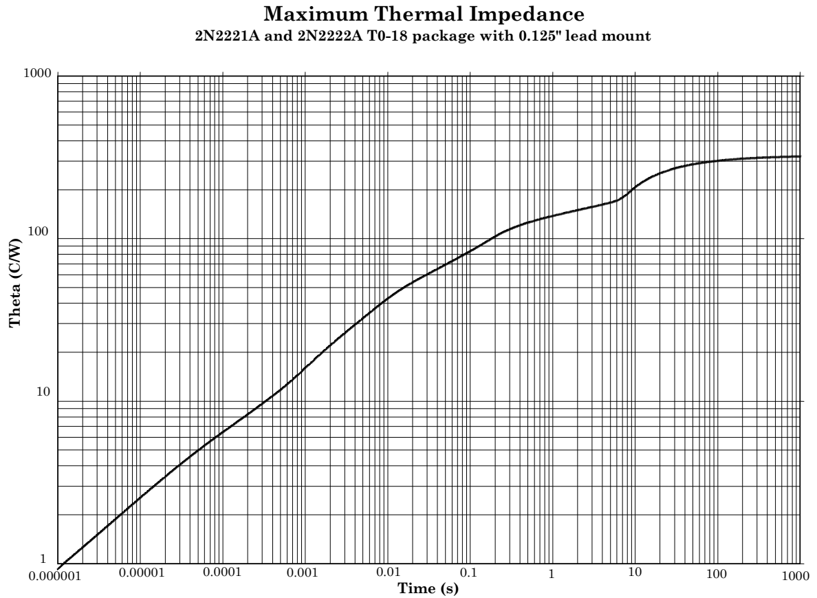
FIGURE 12. Thermal impedance graph ( R_{\theta JA} ) for 2N2221A, 2N2221AL, 2N2222A, and 2N2222AL (TO-18).
