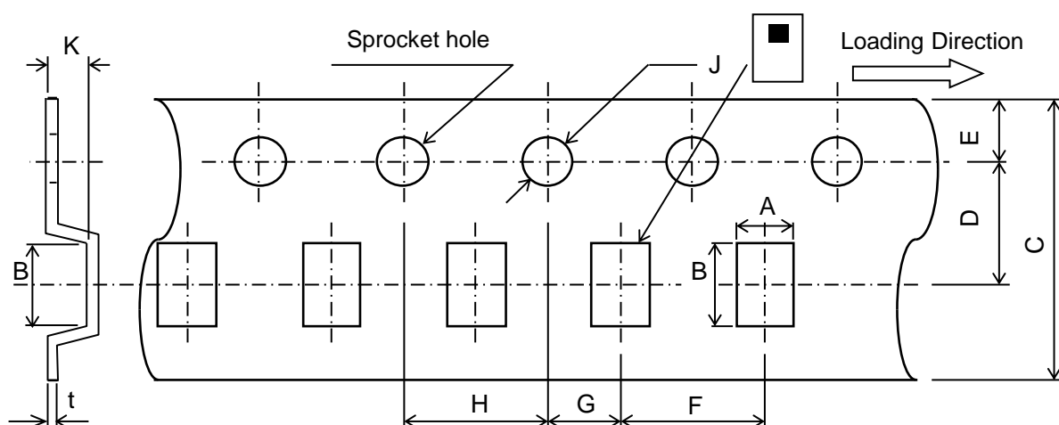
Dimensions (mm)
