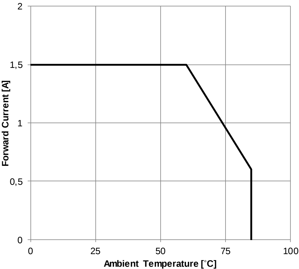
Derating Curve:
