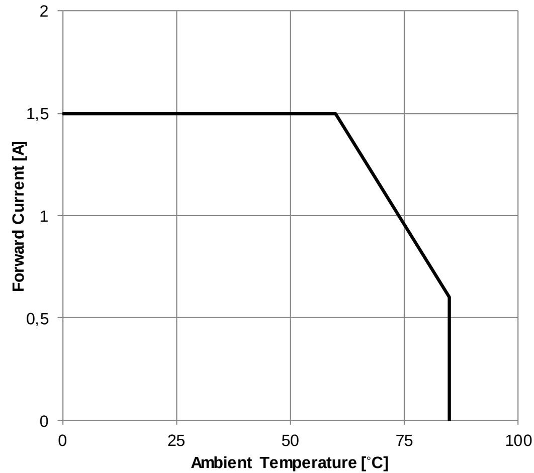
Derating Curve:
