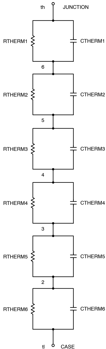
Figure 24. Thermal Model
