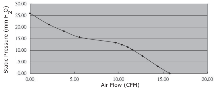
CFM-4028BG-1130-475
