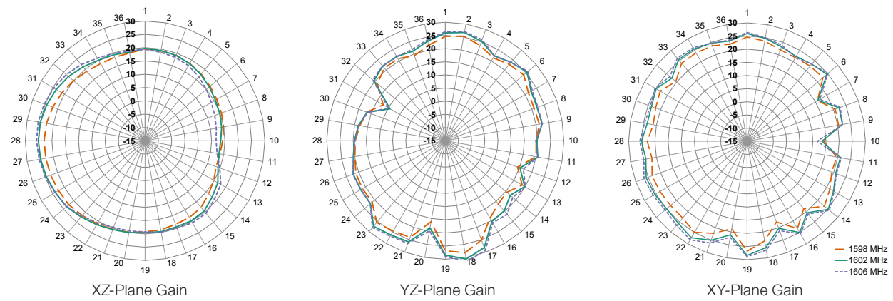
Figure 6. ANT-GNCP-C106L160 Radiation Patterns
