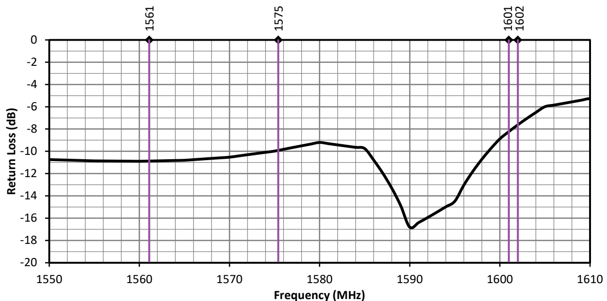
Figure 3. ANT-GNCP-C106L160 Return Loss
