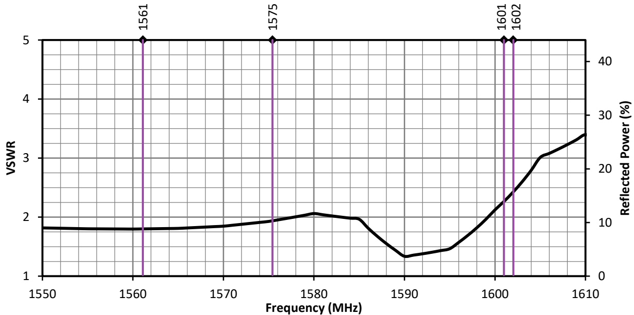
Figure 2. ANT-GNCP-C106L160 VSWR
