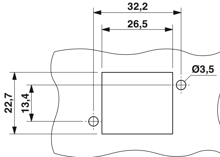
Dimensional drawing
