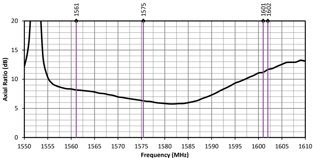
Figure 5. ANT-GNCP-C357L160 Antenna Axial Ratio
