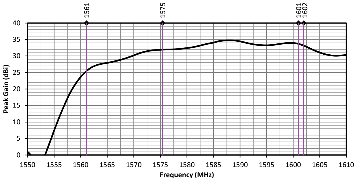
Figure 4. ANT-GNCP-C357L160 Peak Gain
