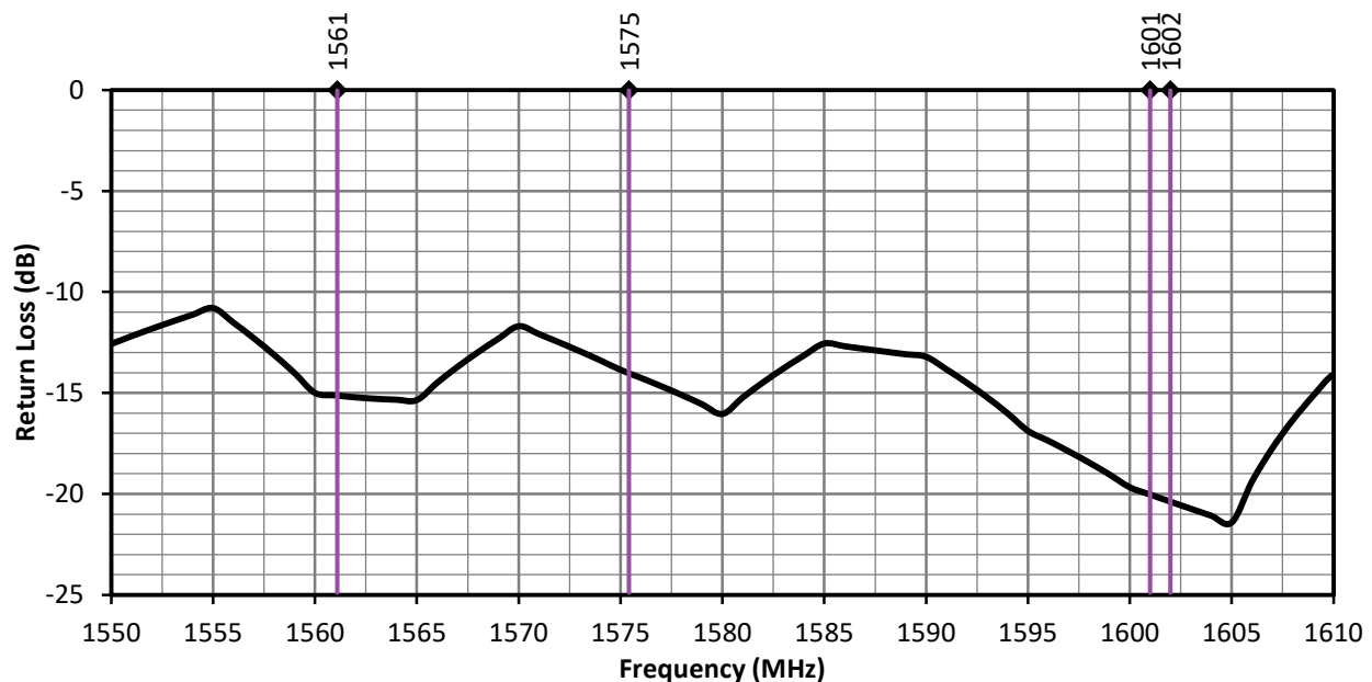
Figure 3. ANT-GNCP-C357L160 Return Loss
