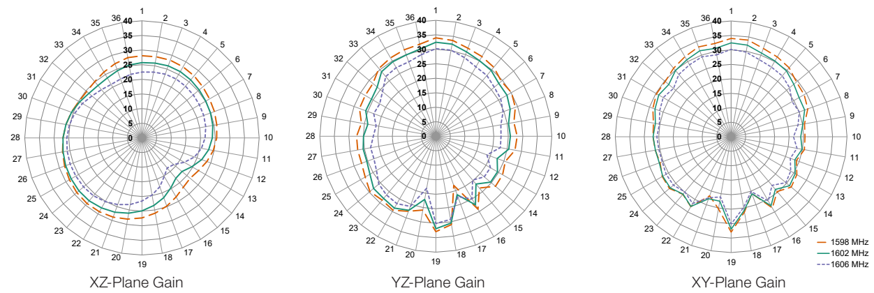
Figure 6. ANT-GNCP-C357L160 Radiation Patterns
