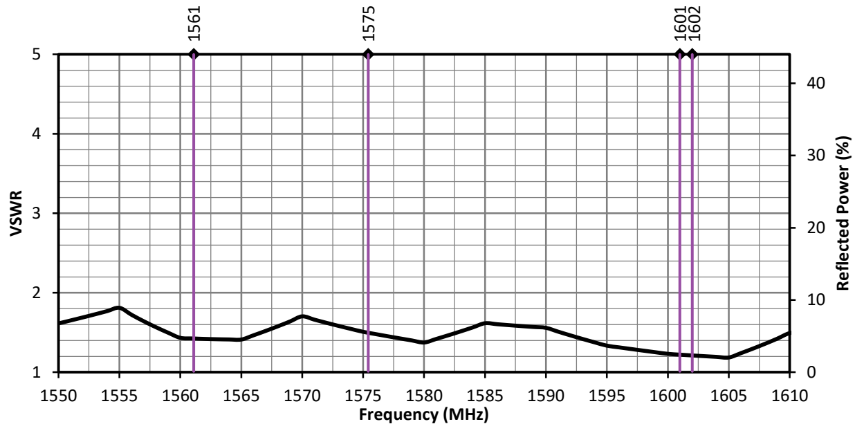
Figure 2. ANT-GNCP-C357L160 VSWR
