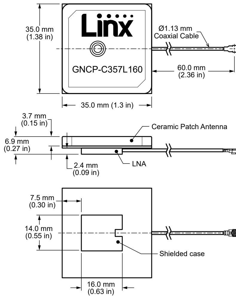
Figure 1. ANT-GNCP-C357L160 Antenna Dimensions
