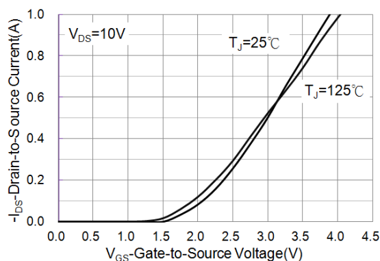
Fig.2 Transfer Characteristics
