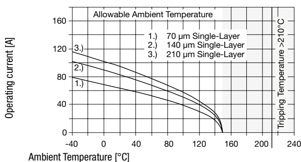
Derating Curve with Shunt (RTS-BS500)
