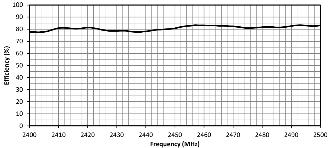
Figure 8. Antenna Radiation Efficiency for ANT-2.4-PW-LPN, Edge of ground Plane
