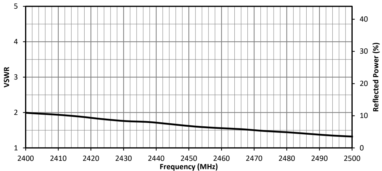
Figure 4. VSWR for ANT-2.4-PW-LPN, Edge of ground Plane
