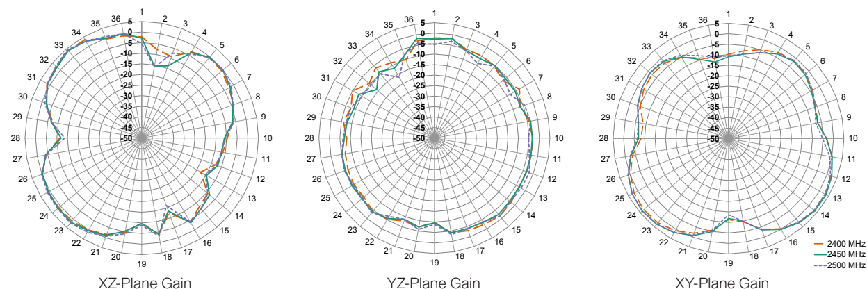
Figure 9. Radiation Patterns for ANT-2.4-PW-LPN Antenna, Edge of ground Plane
