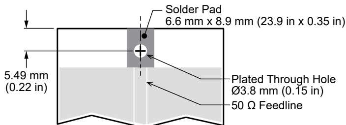
Figure 2. ANT-2.4-PW-LPN Antenna Recommended Mounting and PCB Footprint
