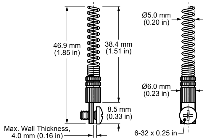
Figure 1. ANT-2.4-PW-LPN Antenna Dimensions
